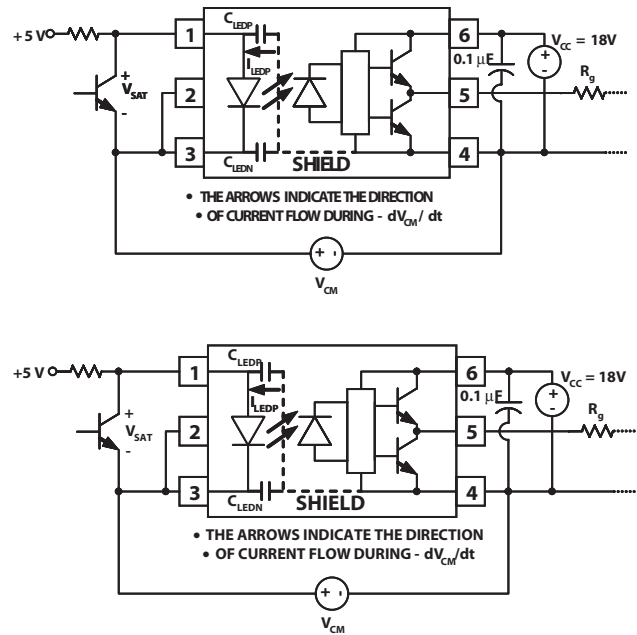
Figure 23. Equivalent Circuit for Figure 17 During Common Mode Transient.
