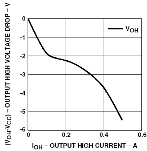
Figure 3. V_{OH} vs. I_{OH} .
