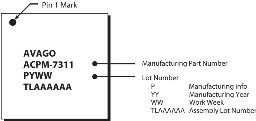
Figure 13. Marking Specifications
