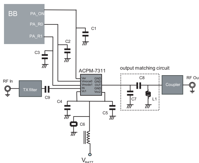
Figure 16. Peripheral Circuits
