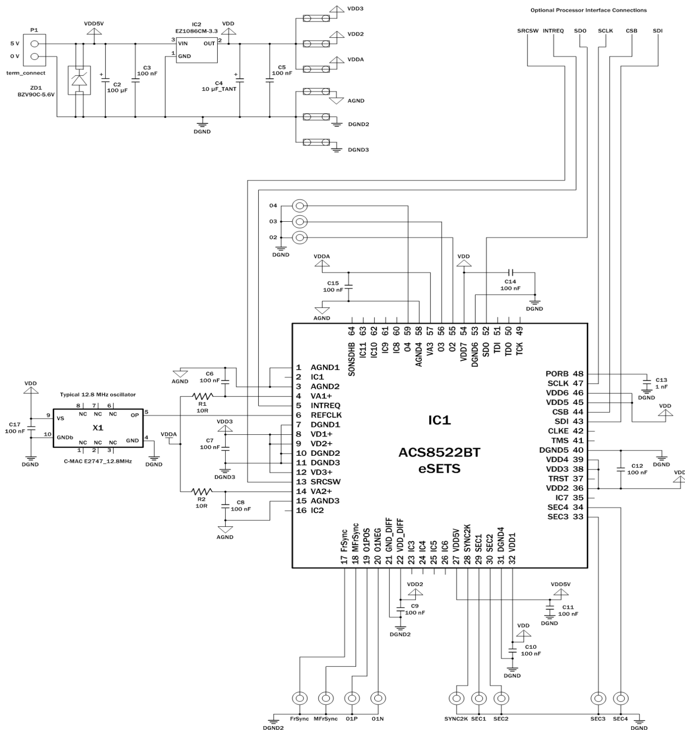
Figure 20 Simplified Application Schematic
