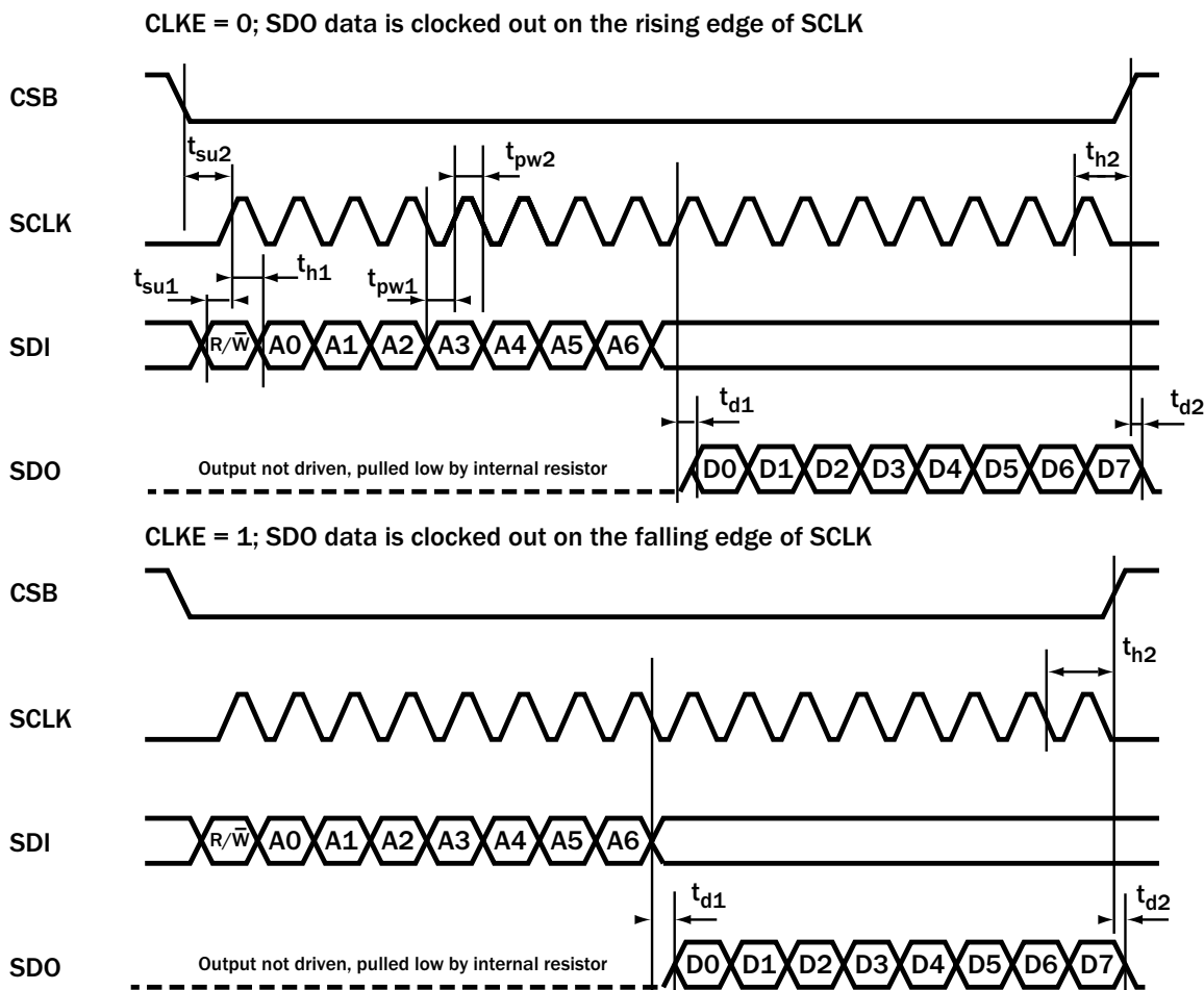
Figure 12 Read Access Timing for SERIAL Interface
