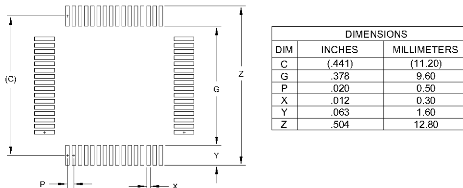
Figure 19 Typical 64 Pin LQFP Footprint
