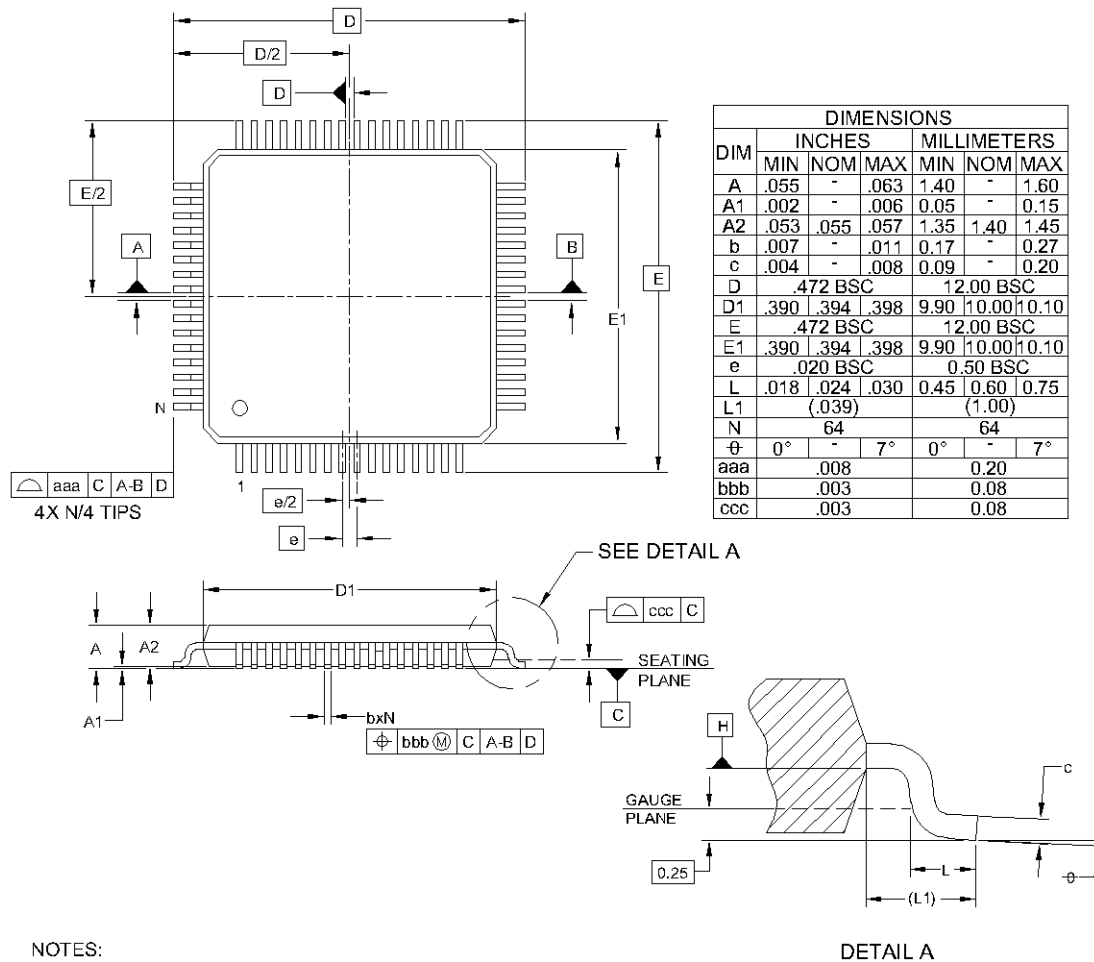
Figure 18 LQFP Package
