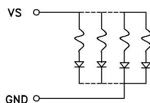
Recommended Set-up
