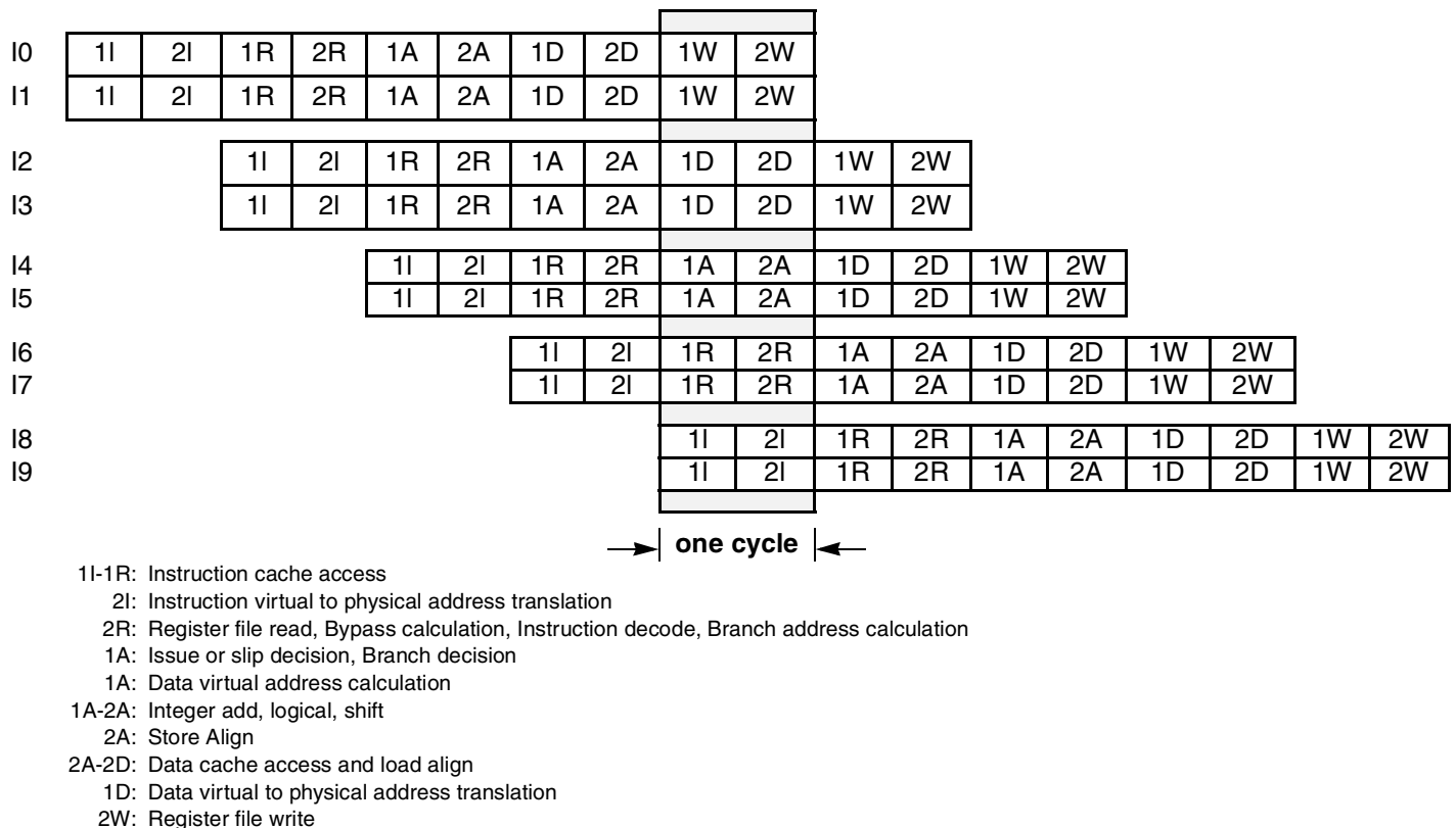
Figure 3 – Pipeline
