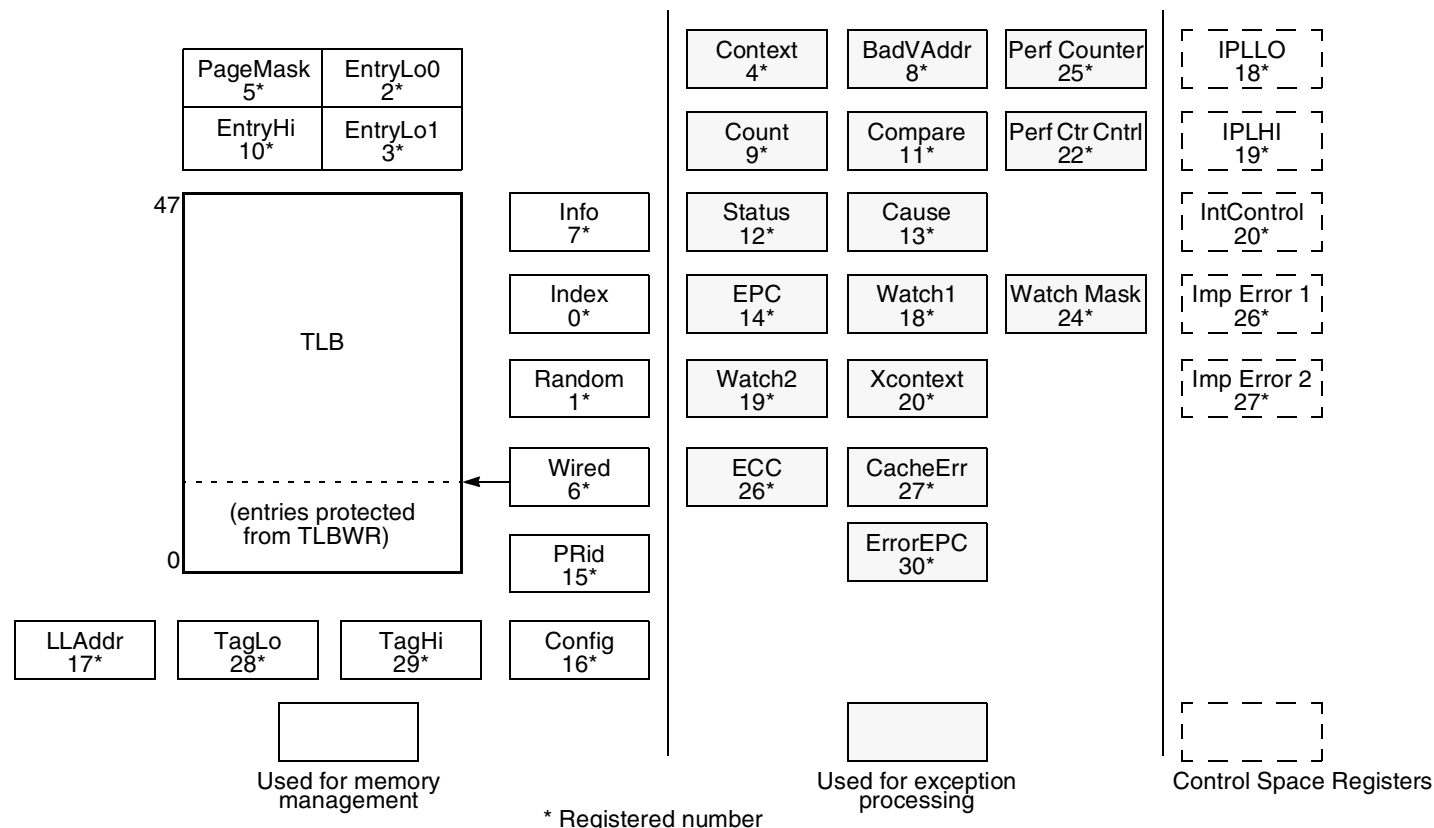
Figure 4 – CP0 Registers
