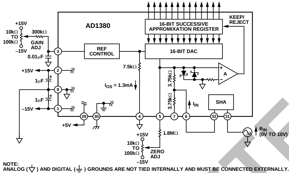
Figure 9. Analog and Power Connections for Unipolar 0 V to 10 V Input Range
