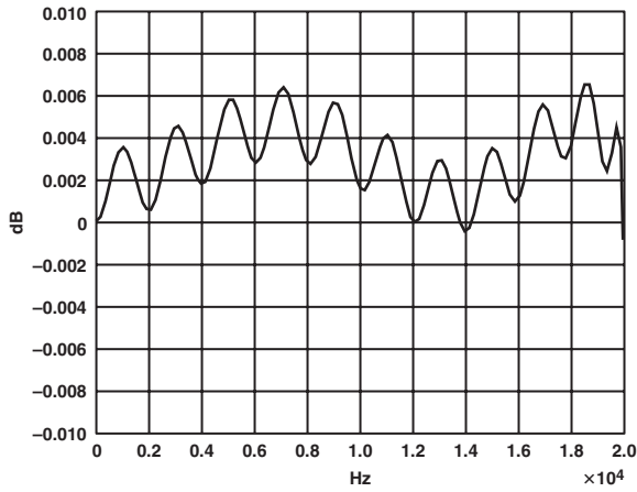
TPC 1. Pass-Band Response, 8× Mode
