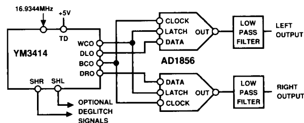
Figure 15. Yamaha YM3414 and AD1856 Interface
