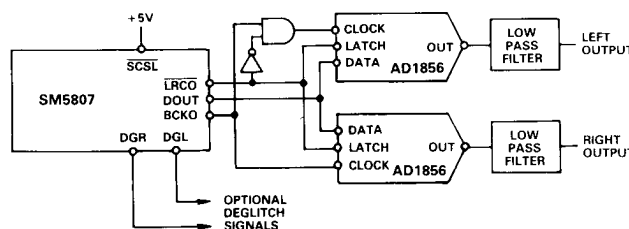
Figure 14. NPC SM5807 and AD1856 Interface
