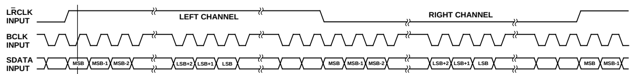
Figure 9. AD1857 Left-Justified Mode
