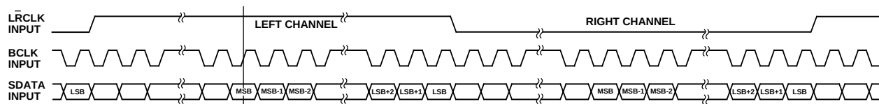
Figure 11. AD1858 Right-Justified Mode
