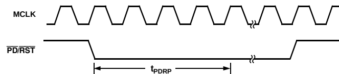
Figure 25. Power-Down/Reset Timing
