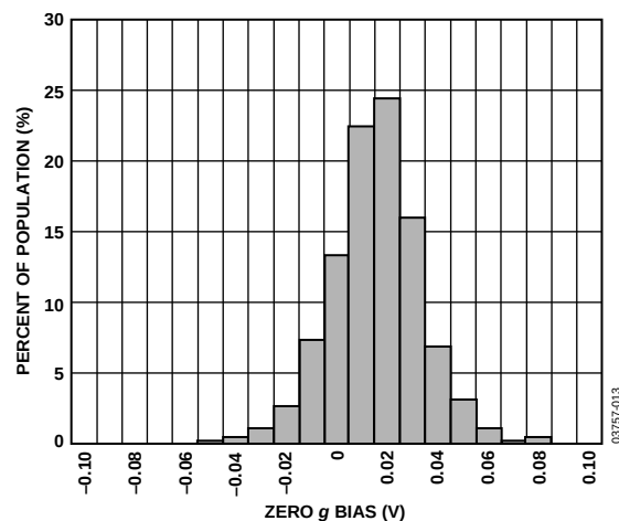
Figure 8. Y-Axis Zero g Bias Deviation from Ideal at 25°C
