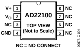
Figure 4. 8-Lead SOIC
