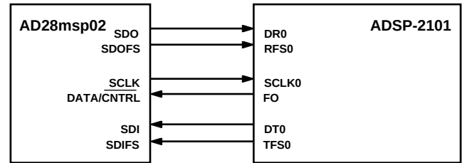
Figure 5. AD28msp02-to-ADSP-2101 Interface
