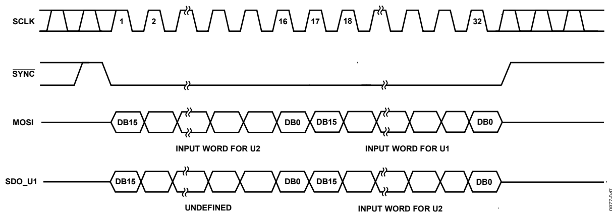
Figure 44. Daisy-Chain Diagram
