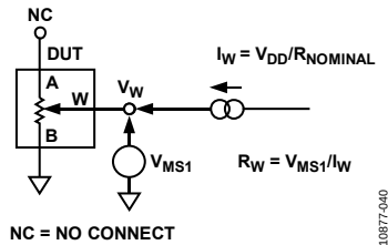
Figure 40. Wiper Resistance
