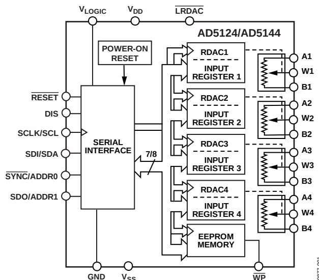
Figure 1. AD5124/AD5144 24-Lead LFCSP
