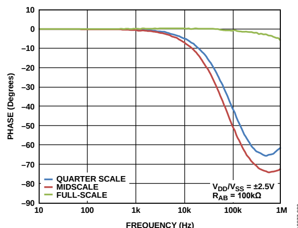
Figure 29. Normalized Phase Flatness vs. Frequency, R_{AB} = 100\text{ k}\Omega
