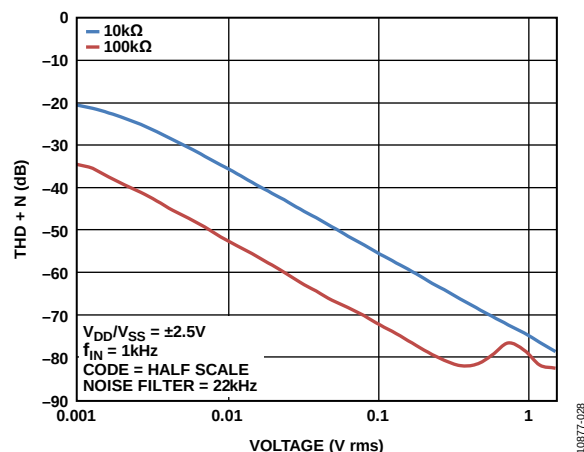
Figure 28. Total Harmonic Distortion Plus Noise (THD + N) vs. Amplitude
