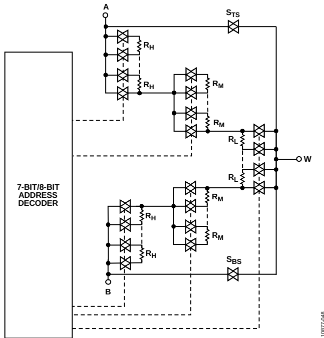
Figure 45. AD5124/AD5144/AD5144A Simplified RDAC Circuit
