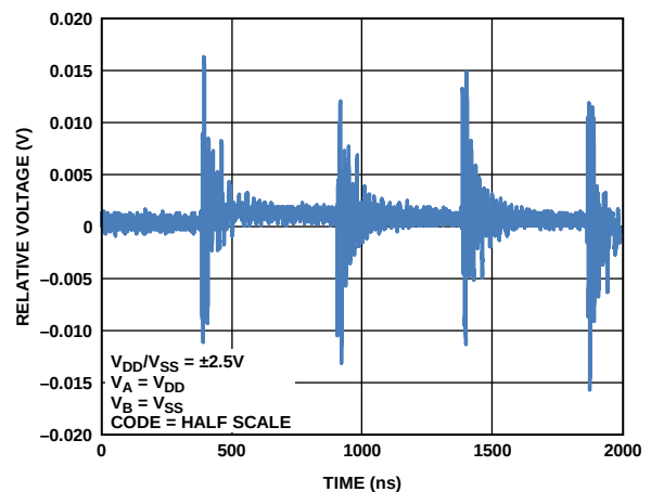
Figure 35. Digital Feedthrough
