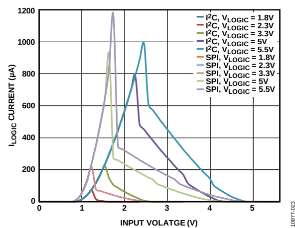
Figure 23. I_{\text{LOGIC}} Current vs. Digital Input Voltage
