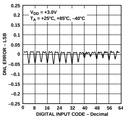
Figure 8. Potentiometer Divider Differential Nonlinearity Error vs. Code
