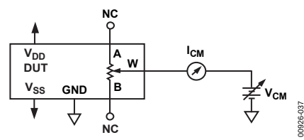
Figure 30. Common-Mode Leakage Current
