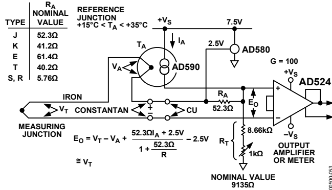
Figure 53. Cold-Junction Compensation
