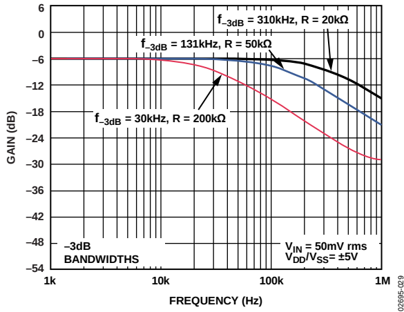
Figure 28. -3 dB Bandwidth
