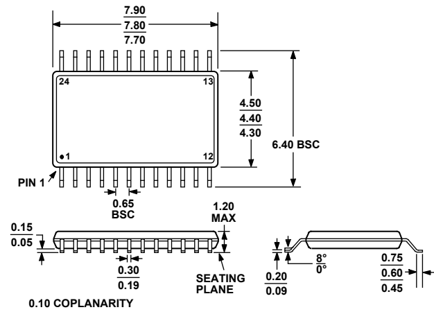
COMPLIANT TO JEDEC STANDARDS MO-153-AD Figure 72. 24-Lead Thin Shrink Small Outline Package [TSSOP] (RU-24) Dimensions shown in millimeters
