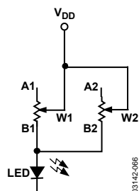
Figure 67. Reduce Resistance by Half with Linear Adjustment Characteristics
