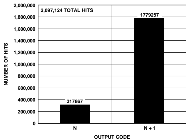
Figure 15. AD6673-250 Grounded Input Histogram
