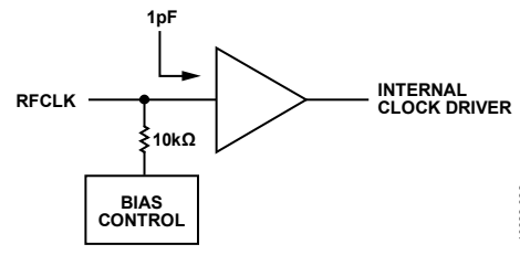
Figure 37. Equivalent RF Clock Input Circuit
