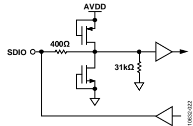
Figure 20. Equivalent SDIO Circuit
