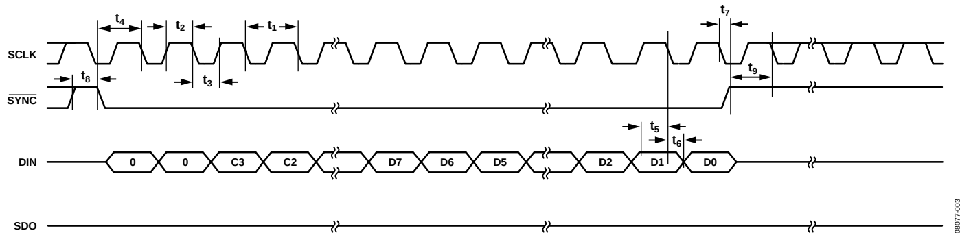
Figure 3. Write Timing Diagram ( CPOL = 0 , CPHA = 1 )
