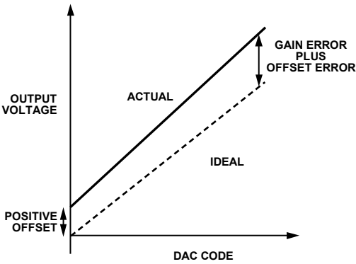
Figure 29. Transfer Function with Positive Offset
