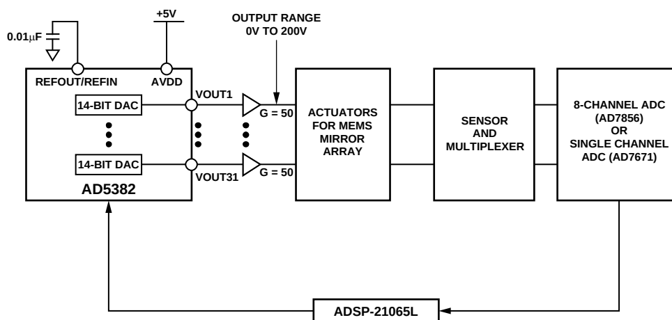
Figure 46. AD5382 in a MEMS Based Optical Switch
