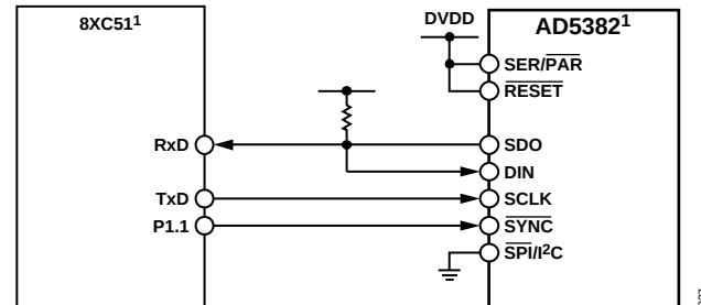
Figure 36. AD5382-to-8051 Interface
