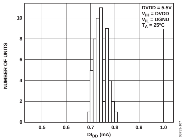
Figure 15. D_{IDD} Histogram
