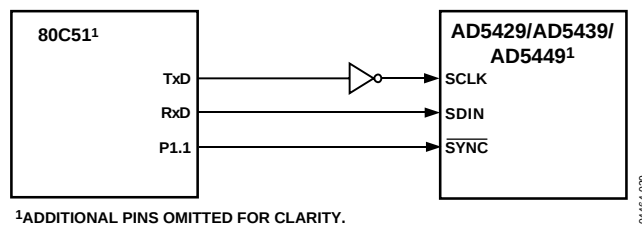
Figure 51. 80C51/80L51-to-AD5429/AD5439/AD5449 Interface
