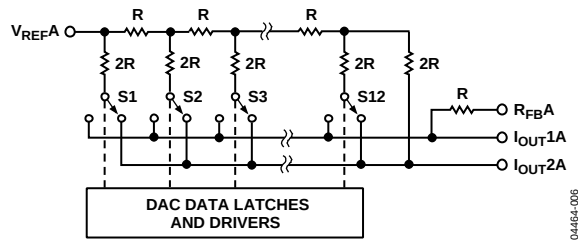
Figure 36. Simplified Ladder
