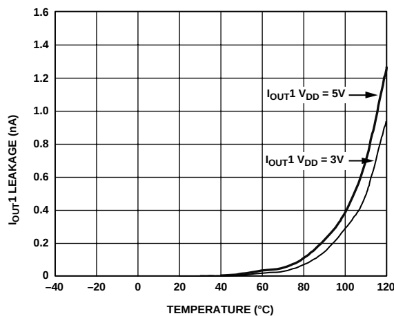
Figure 16. I_{OUT1} Leakage Current vs. Temperature
