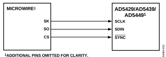
Figure 53. MICROWIRE-to-AD5429/AD5439/AD5449 Interface
