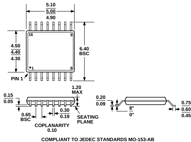
Figure 59. 16-Lead Thin Shrink Small Outline Package [TSSOP] (RU-16) Dimensions shown in millimeters
