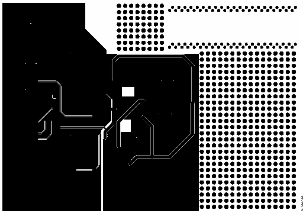
Figure 58. Solder-Side Artwork
