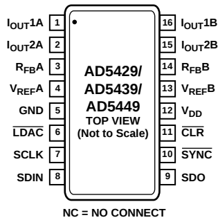
Figure 5. Pin Configuration
