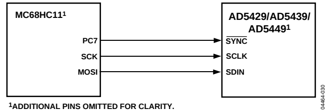
Figure 52. MCH68HC11/68L11-to-AD5429/AD5439/AD5449 Interface
