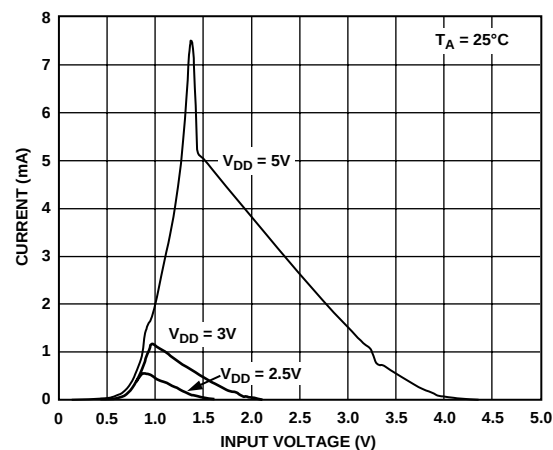
Figure 15. Supply Current vs. Logic Input Voltage
