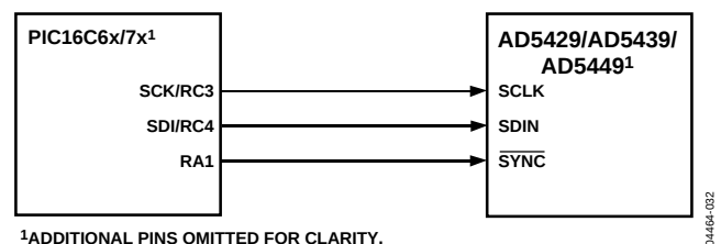
Figure 54. PIC16C6x/7x-to-AD5429/AD5439/AD5449 Interface
