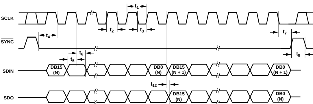
Figure 2. Standalone Mode Timing Diagram
