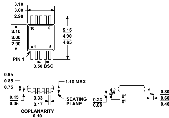
COMPLIANT TO JEDEC STANDARDS MO-187-BA Figure 58. 10-Lead Mini Small Outline Package [MSOP] (RM-10) Dimensions shown in millimeters
