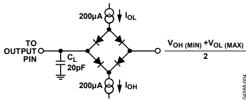
Figure 4. Load Circuit for SDO Timing Specifications
