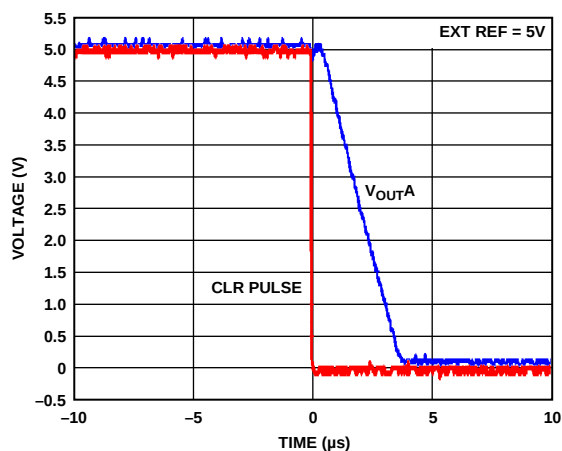
Figure 44. Hardware \overline{\text{CLR}}
