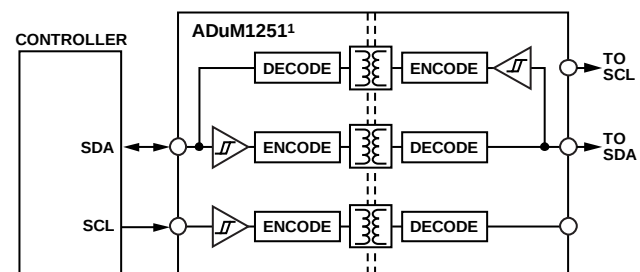
Figure 70. Isolated Interface
