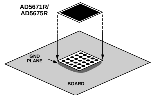
Figure 69. Pad Connection to Board
