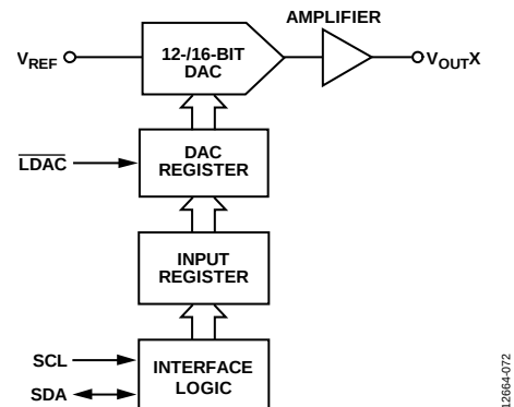
Figure 63. Simplified Diagram of Input Loading Circuitry for a Single DAC
