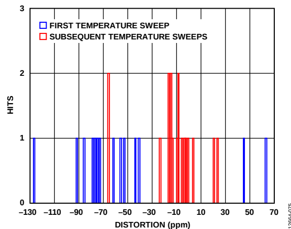
Figure 66. Thermal Hysteresis
