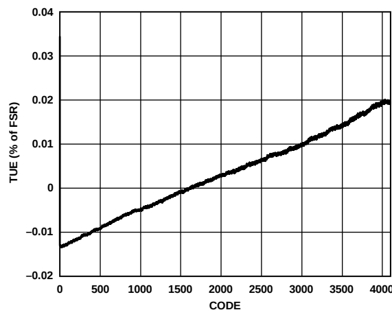
Figure 11. AD5671R TUE vs. Code
