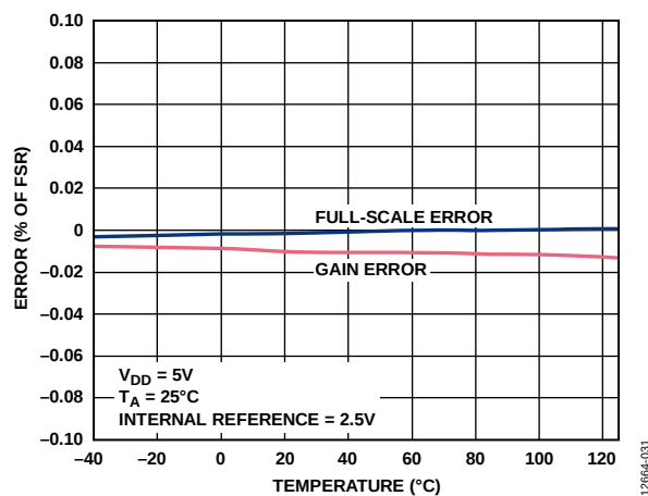
Figure 23. AD5675R Gain Error and Full-Scale Error vs. Temperature
