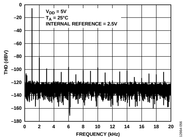
Figure 47. Total Harmonic Distortion (THD) at 1 kHz
