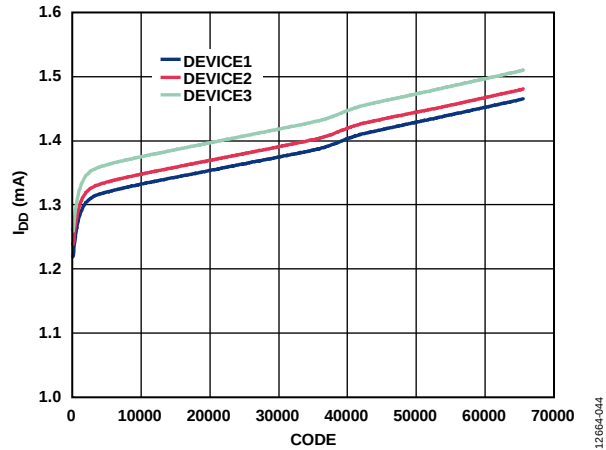
Figure 35. Supply Current ( I_{DD} ) vs. Code
