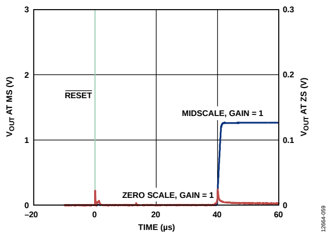
Figure 50. Hardware Reset
