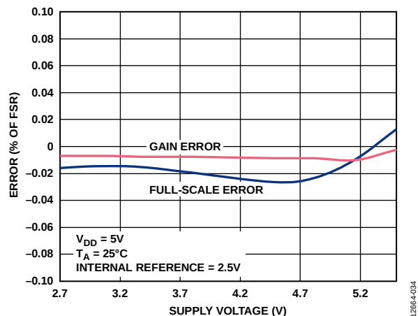
Figure 26. AD5671R Gain Error and Full-Scale Error vs. Supply Voltage
