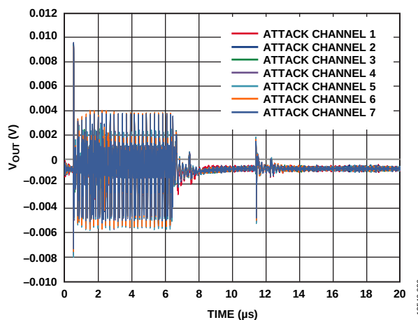
Figure 33. DAC-to-DAC Crosstalk
