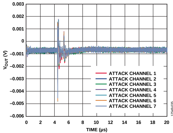
Figure 32. Analog Crosstalk
