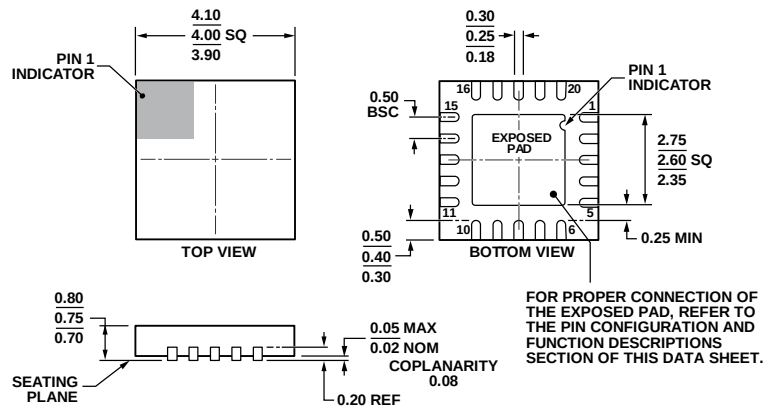
Figure 53. 20-Lead Lead Frame Chip Scale Package [LFCSP] 4 mm × 4 mm Body and 0.75 mm Package Height (CP-20-8)
