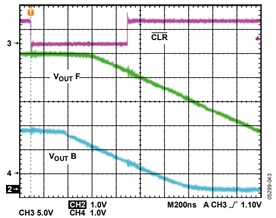
Figure 43. Hardware \overline{CLR}
