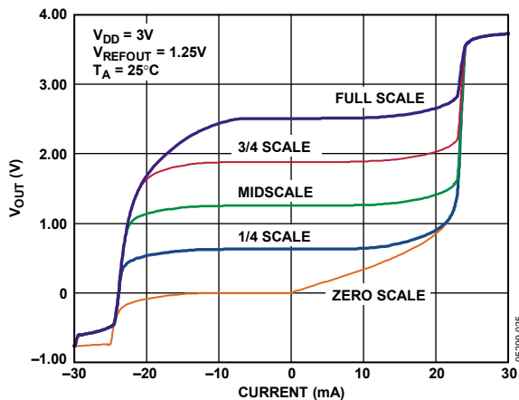
Figure 25. AD5678-1 Source and Sink Capability
