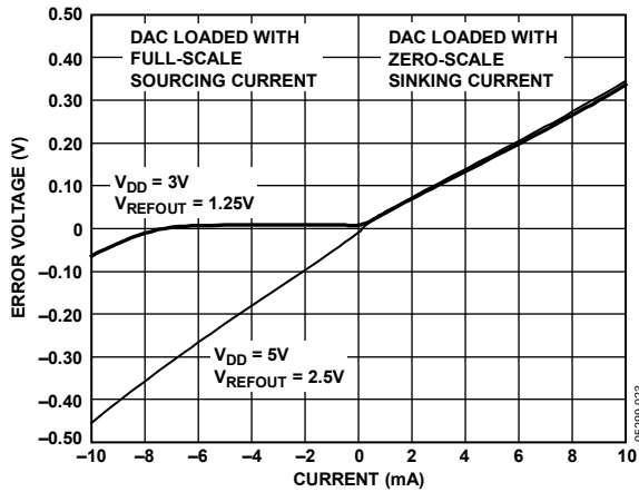
Figure 23. Headroom at Rails vs. Source and Sink
