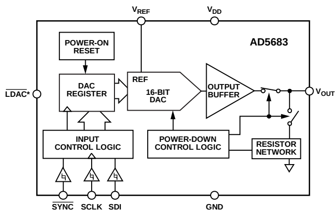
Figure 3. AD5683 LFCSP
