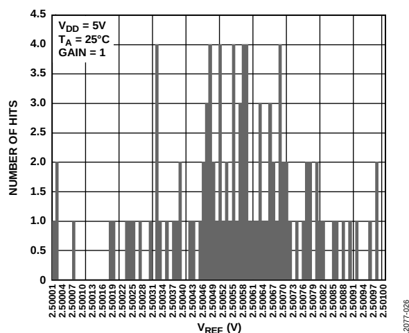
Figure 26. Reference Output Spread
