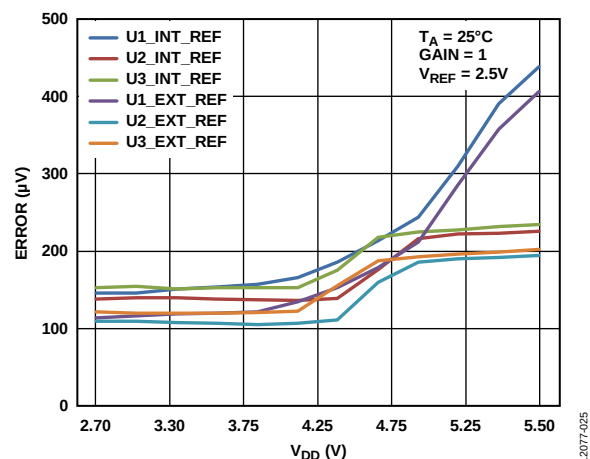
Figure 25. Zero Code Error and Offset Error vs. V_{DD}
