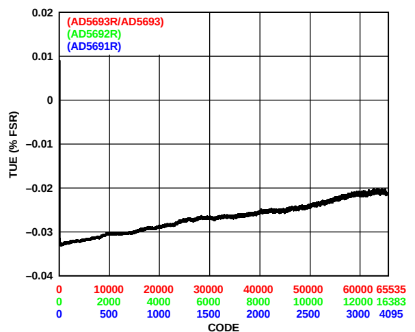
Figure 19. TUE vs. Code
