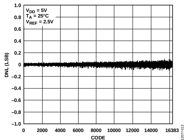
Figure 13. AD5692R DNL
