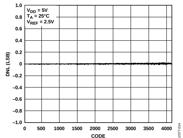
Figure 14. AD5691R DNL
