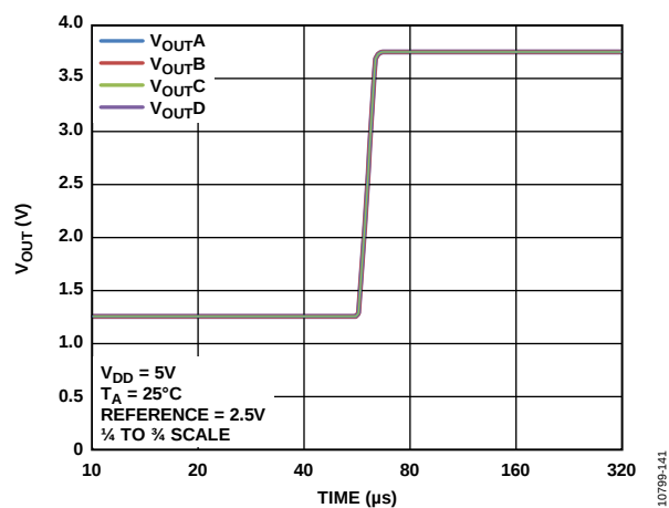
Figure 24. Settling Time
