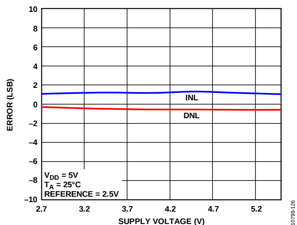
Figure 11. INL Error and DNL Error vs. Supply Voltage
