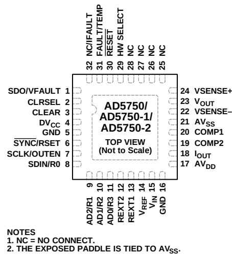
Figure 4. Pin Configuration
