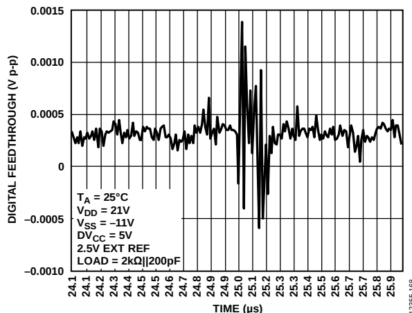
Figure 70. Digital Feedthrough
