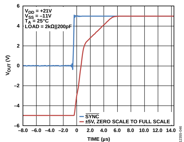
Figure 48. Full-Scale Settling Time (Rising Voltage Step), \pm 5 V Range
