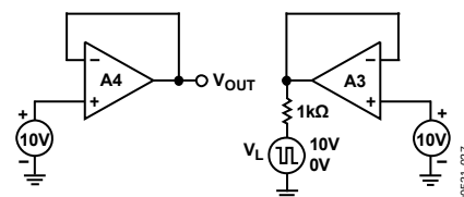
Figure 27. Load Crosstalk Test Circuit
