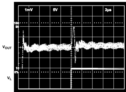
Figure 28. Load Crosstalk
