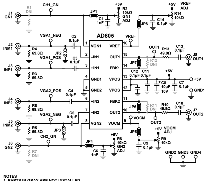
Figure 43. Schematic Diagram of the AD605-EVALZ Evaluation Board
