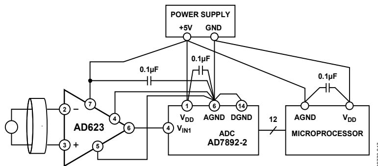
Figure 48. Optimal Ground Practice in a Single-Supply Environment
