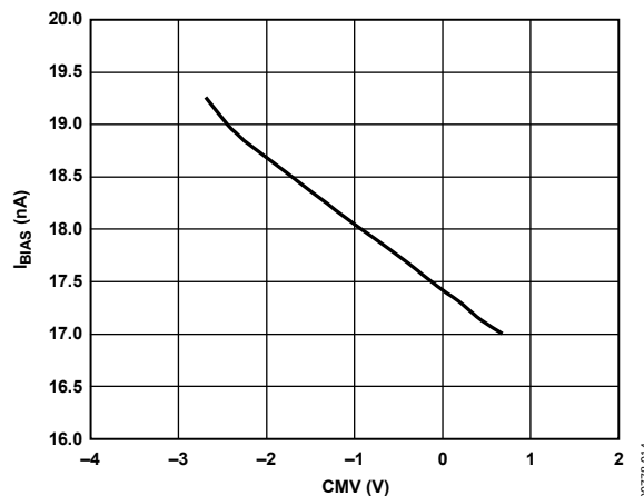
Figure 14. I_{BIAS} vs. CMV, V_S = \pm 2.5 V
