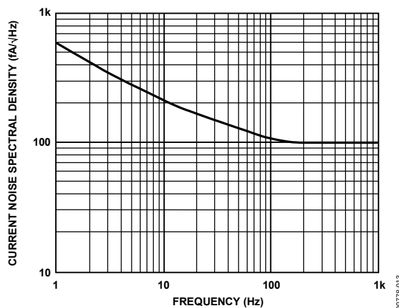
Figure 13. Current Noise Spectral Density vs. Frequency
