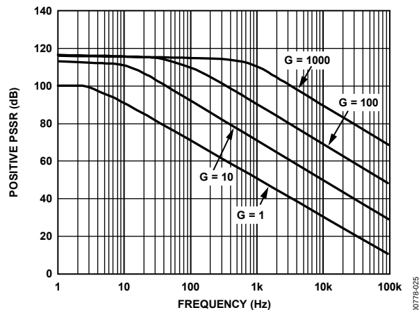
Figure 25. Positive PSRR vs. Frequency, +V_S = 5 \text{ V} , -V_S = 0 \text{ V} , for Various Gain Settings ( G )
