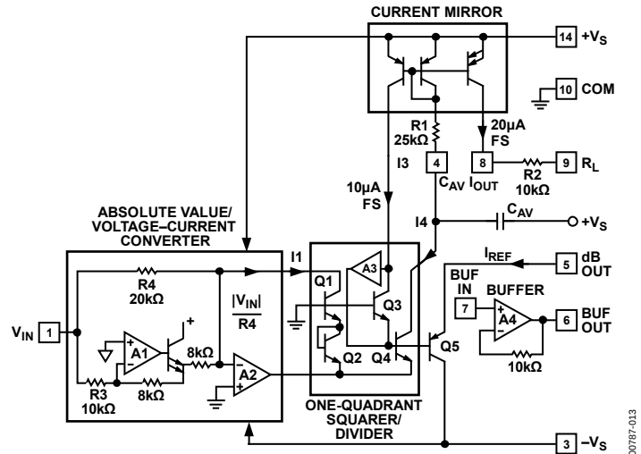
Figure 7. Simplified Schematic
