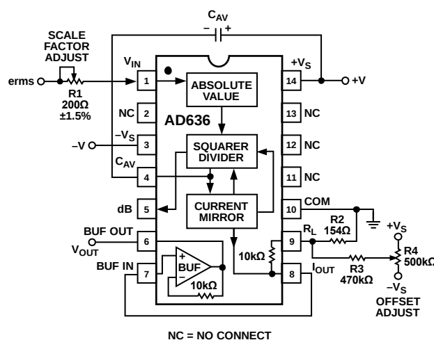
Figure 10. Optional External Gain and Output Offset Trims
