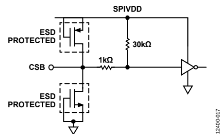
Figure 68. SCLK Inputs
