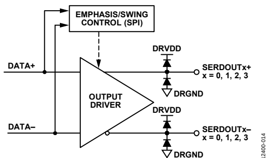
Figure 66. Digital Outputs
