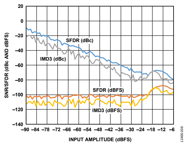
Figure 21. Two-Tone IMD3/SFDR vs. Input Amplitude ( A_{IN} ) with f_{IN1} = 338\text{ MHz} and f_{IN2} = 341\text{ MHz}
