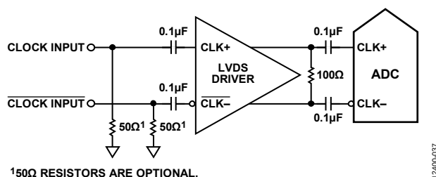
Figure 92. Differential LVDS Sample Clock
