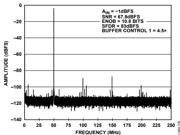
Figure 47. Single Tone FFT with f_{IN} = 450.3 MHz
