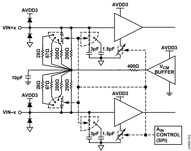
Figure 63. Analog Inputs
