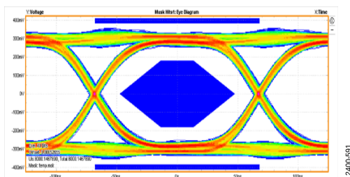
Figure 132. Digital Output Data Eye, External 100 \Omega Terminations at 7.37 Gbps
