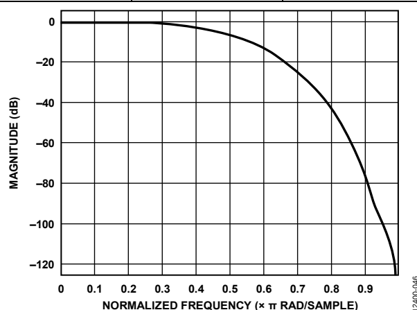
Figure 107. HB3 Filter Response
