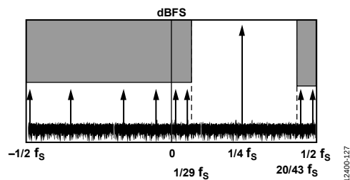
Figure 122. 43% VDR Bandwidth, Complex Mode
