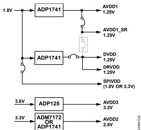
Figure 145. High Efficiency, Low Noise Power Solution for the AD6674
