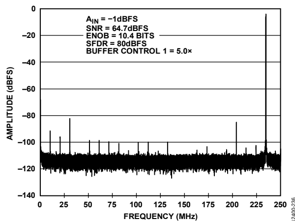
Figure 48. Single Tone FFT with f_{IN} = 765.3 MHz
