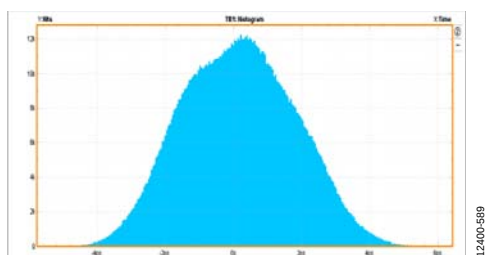
Figure 130. Histogram, External 100 \Omega Terminations at 10 Gbps
