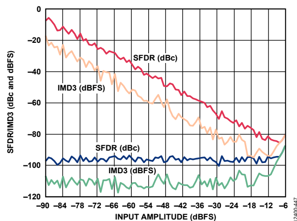
Figure 58. Two-Tone SFDR/IMD3 vs. Input Amplitude ( A_{IN} ) with f_{IN1} = 184\text{ MHz} and f_{IN2} = 187\text{ MHz}
