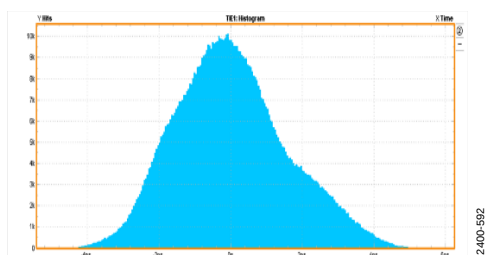
Figure 133. Histogram, External 100 \Omega Terminations at 7.37 Gbps
