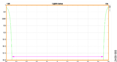
Figure 134. Bathtub, External 100 \Omega Terminations at 7.37 Gbps
