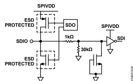
Figure 69. CSB Input
