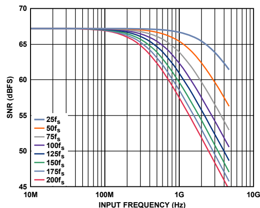
Figure 95. Estimated SNR Degradation for the AD6674-1000 vs. Input Frequency and Jitter
