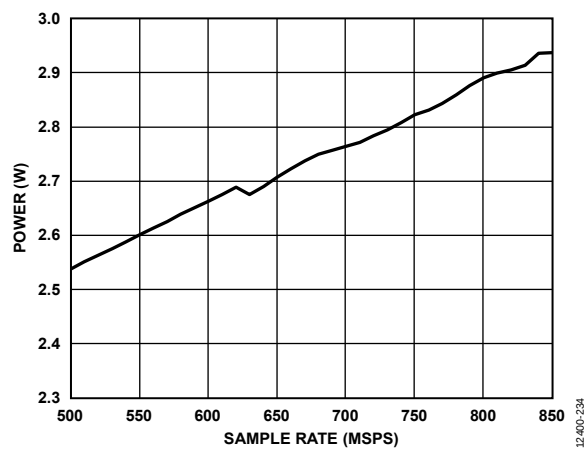
Figure 43. Power Dissipation vs. Sample Rate ( f_s ); L = 4 , M = 2 , F = 1 for f_s \geq 625 MSPS and L = 2 , M = 2 , F = 2 for f_s < 625 MSPS (Default SPI)
