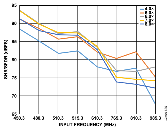
Figure 85. Buffer Current Sweeps, AD6674-500 (SFDR vs. Input Frequency and I_{BUFF} ); 450\text{ MHz} < f_{IN} < 1000\text{ MHz} ; Front-End Network Shown in Figure 74
