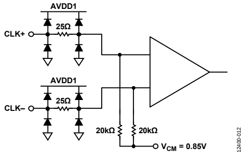
Figure 64. Clock Inputs
