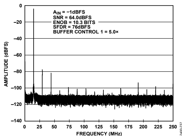
Figure 49. Single Tone FFT with f_{IN} = 985.3 MHz
