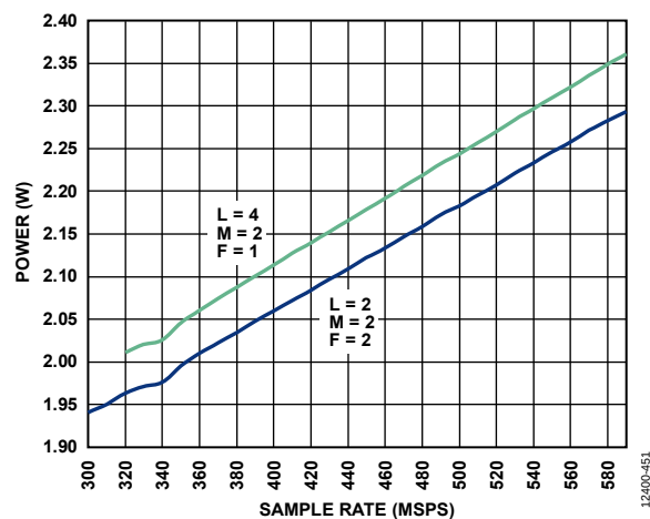
Figure 62. Power Dissipation vs. Sample Rate ( f_s ) (Default SPI)
