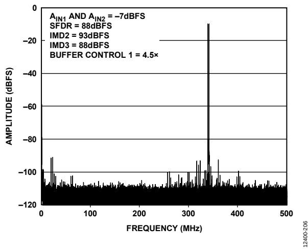
Figure 19. Two-Tone FFT; f_{IN1} = 338\text{ MHz} , f_{IN2} = 341\text{ MHz}
