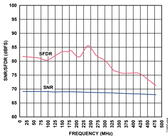
Figure 55. SNR/SFDR vs. Analog Input Frequency ( f_{IN} ); f_{IN} < 500 MHz; Buffer Control 1 = 3.0x
