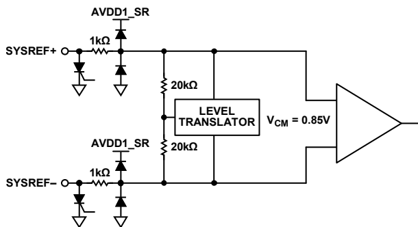
Figure 65. SYSREF± Inputs
