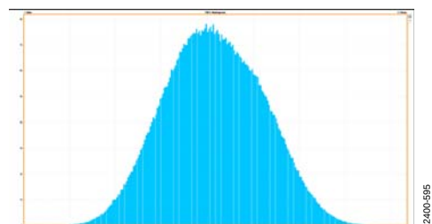
Figure 136. Histogram, External 100 \Omega Terminations at 6 Gbps
