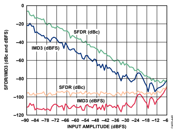
Figure 59. Two-Tone SFDR/IMD3 vs. Input Amplitude ( A_{IN} ) with f_{IN1} = 338\text{ MHz} and f_{IN2} = 341\text{ MHz}
