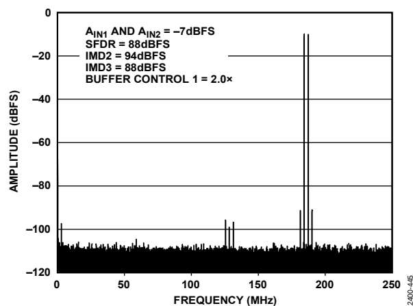
Figure 56. Two-Tone FFT; f_{IN1} = 184\text{ MHz} , f_{IN2} = 187\text{ MHz}
