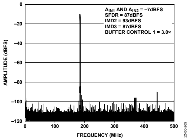
Figure 18. Two-Tone FFT; f_{IN1} = 184\text{ MHz} , f_{IN2} = 187\text{ MHz}
