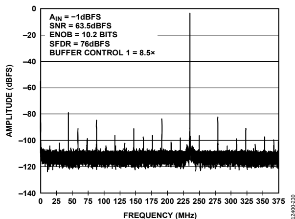
Figure 30. Single Tone FFT with f_{IN} = 985.3 MHz
