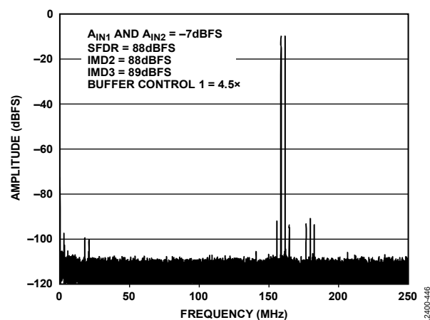
Figure 57. Two-Tone FFT; f_{IN1} = 338\text{ MHz} , f_{IN2} = 341\text{ MHz}
