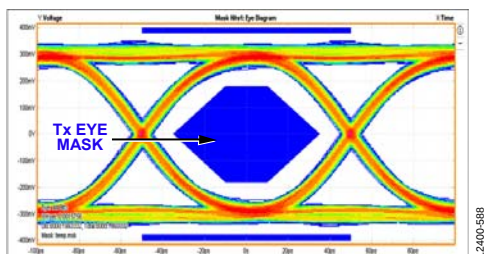
Figure 129. Digital Output Data Eye, External 100 \Omega Terminations at 10 Gbps
