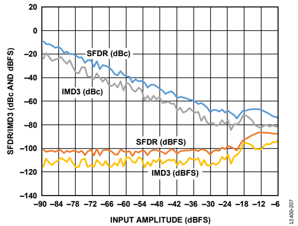
Figure 20. Two-Tone SFDR/IMD3 vs. Input Amplitude ( A_{IN} ) with f_{IN1} = 184\text{ MHz} and f_{IN2} = 187\text{ MHz}
