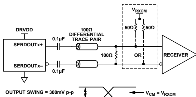
Figure 127. AC-Coupled Digital Output Termination Example
