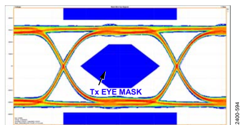
Figure 135. Digital Output Data Eye, External 100 \Omega Terminations at 6 Gbps
