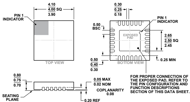
Figure 67. 24-Lead Lead Frame Chip Scale Package [LFCSP_WQ] 4 mm x 4 mm Body, Very Very Thin Quad (CP-24-7)
