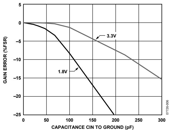
Figure 6. Capacitance Input Gain Error vs. Capacitance C_{IN} to GND, V_{DD} = 1.8V and 3.3V , C_{IN} to EXC = 9pF
