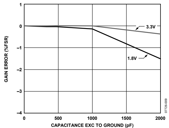
Figure 9. Capacitance Input Gain Error vs. Capacitance C_{EXC} to GND, V_{DD} = 1.8V and 3.3V , C_{IN} to EXC = 9pF
