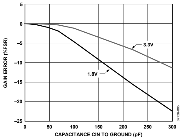
Figure 5. Capacitance Input Gain Error vs. Capacitance C_{IN} to GND, V_{DD} = 1.8V and 3.3V , C_{IN} to EXC = 3pF
