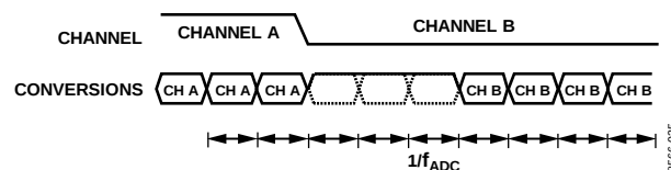
Figure 36. Sinc 3 Channel Change
