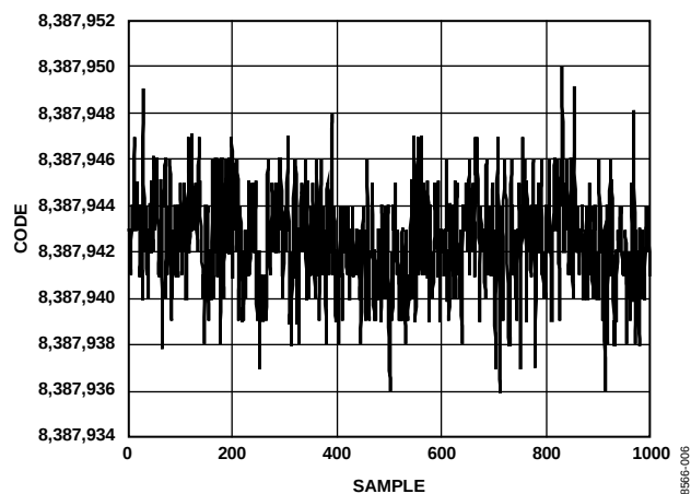
Figure 6. Noise ( V_{REF} = AV_{DD} = 5\text{ V} , Output Data Rate = 4.7 Hz, Gain = 128, Chop Disabled, Sinc 4 Filter)
