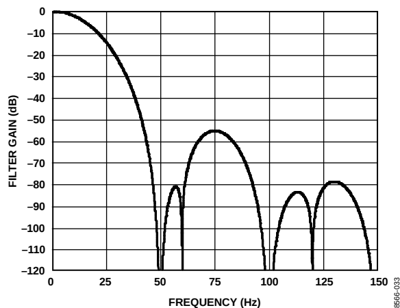
Figure 34. Sinc 4 Filter Response (FS[9:0] = 96, REJ60 = 1)
