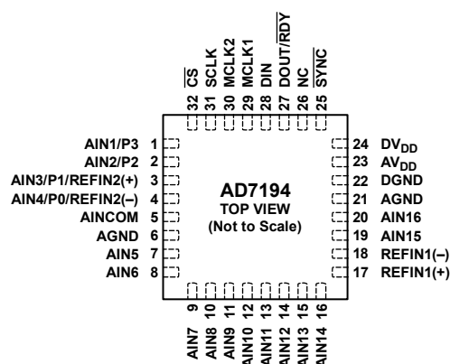
Figure 5. Pin Configuration
