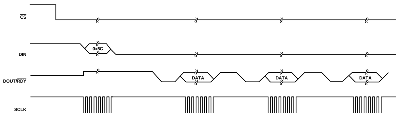
Figure 26. Continuous Read
