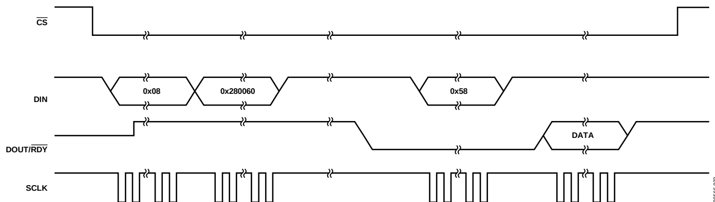
Figure 24. Single Conversion
