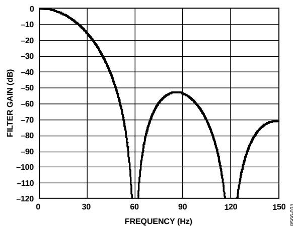
Figure 32. \text{Sinc}^4 Filter Response (FS[9:0] = 80)
