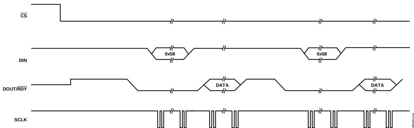
Figure 25. Continuous Conversion
