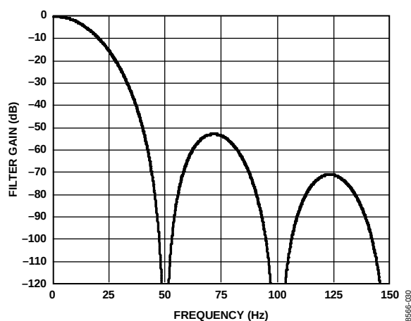
Figure 31. \text{Sinc}^4 Filter Response (FS[9:0] = 96)
