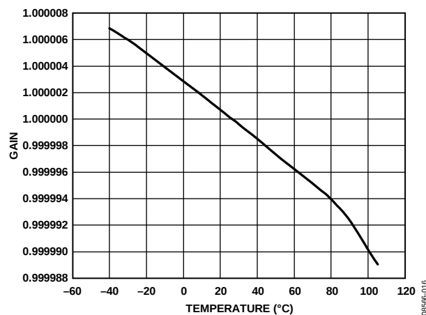
Figure 16. Gain vs. Temperature (Gain = 1)
