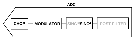
Figure 43. Chop Enabled
