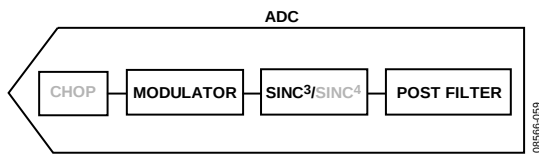
Figure 60. Fast Settling Mode, Sinc 3 Filter
