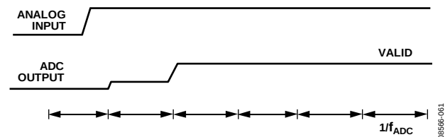
Figure 62. Step Change on Analog Input, Sinc 3 Filter
