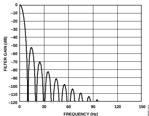
Figure 33. \text{Sinc}^4 Filter Response (FS[9:0] = 480)
