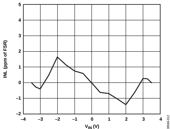
Figure 12. INL (Gain = 1)
