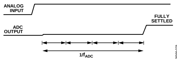
Figure 30. \text{Sinc}^4 Zero Latency Operation
