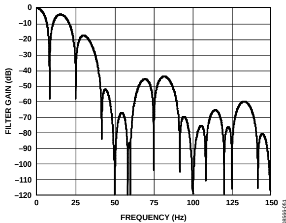
Figure 52. \text{Sinc}^3 Filter Response (FS[9:0] = 96, Chop Enabled, REJ60 = 1)
