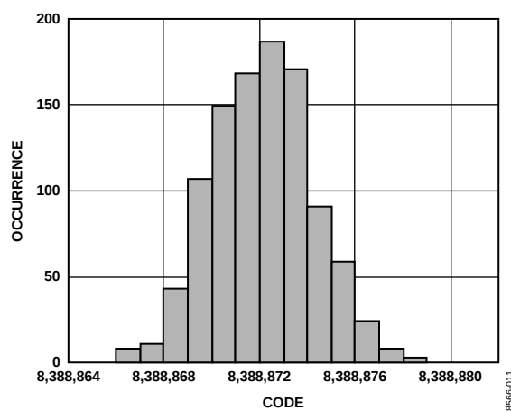
Figure 11. Noise Distribution Histogram ( V_{REF} = AV_{DD} = 5\text{ V} , Output Data Rate = 42.1 Hz (FS[9:0] = 6, Average by 16), Gain = 1, Chop Disabled, Sinc 4 Filter)
