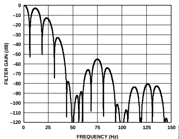
Figure 47. Sinc 4 Filter Response (FS[9:0] = 96, Chop Enabled, REJ60 = 1)
