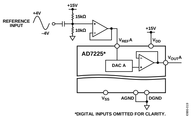
Figure 19. Applying an AC Signal to the AD7225
