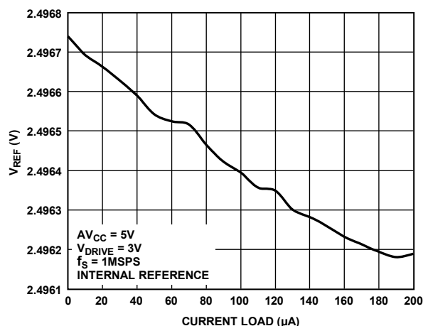
Figure 14. V_{REF} vs. Reference Output Current Drive
