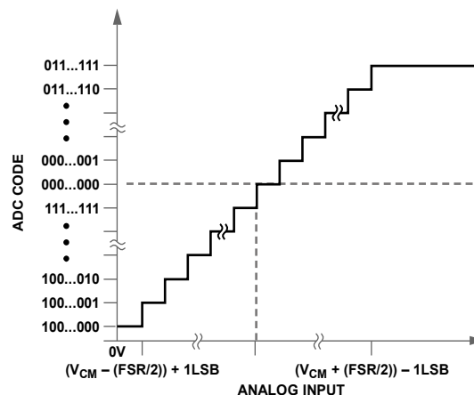
Figure 25. Twos Complement Transfer Function
