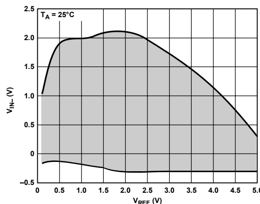
Figure 29. V_{IN-} Input Voltage Range vs. V_{REF} in Pseudo Differential Mode with V_{DD} = 5 \text{ V}
