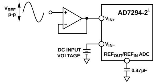
Figure 37. Pseudo Differential Mode Connection Diagram
