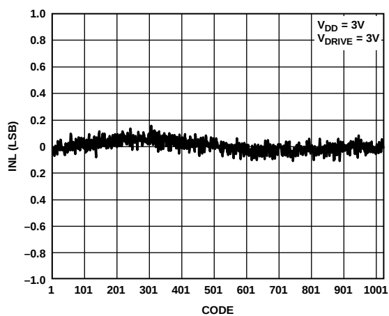
Figure 4. Typical ADC INL
