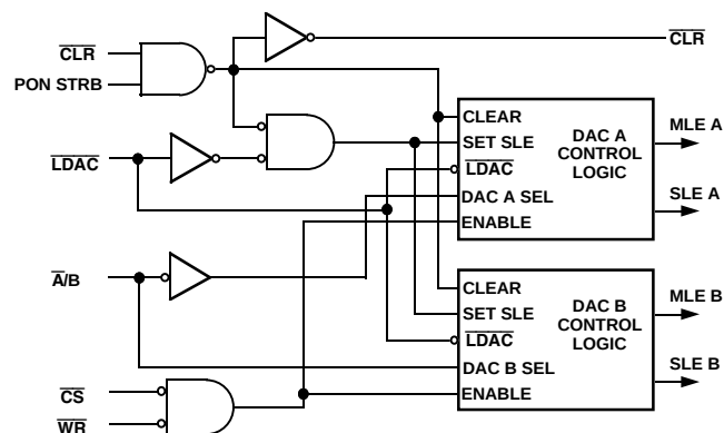
Figure 21. Logic Interface
