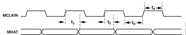
Figure 3. Data Timing
