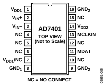
Figure 5. Pin Configuration
