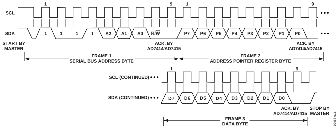
Figure 11. Writing to the Address Pointer Register Followed by a Single Byte of Data to the Selected Register
