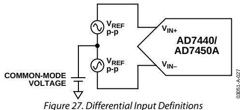
Figure 27. Differential Input Definitions
